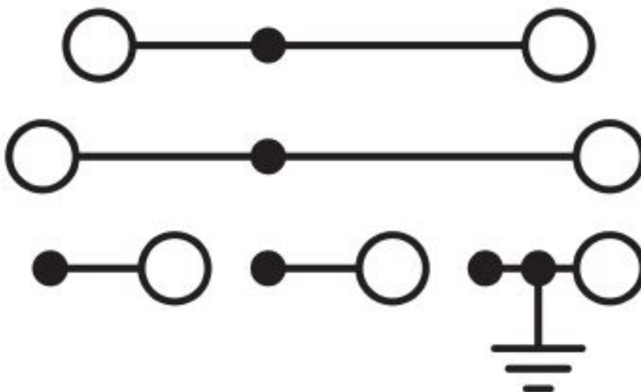
Circuit diagram
