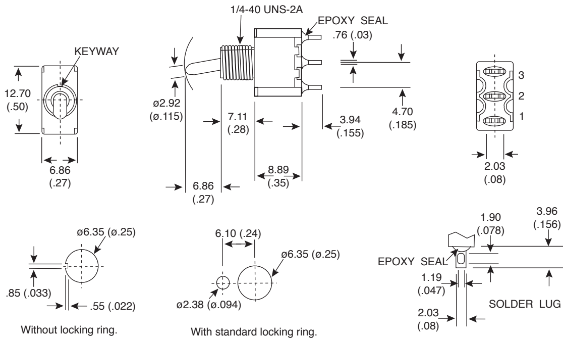
PANEL MOUNTING
