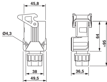
Dimensional drawing
