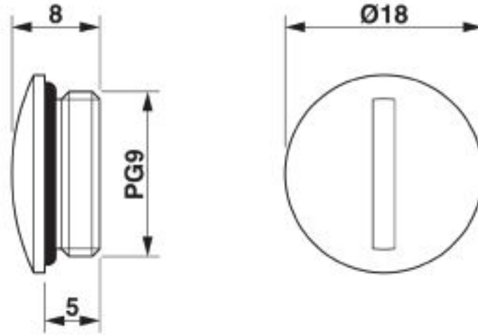
Dimensional drawing
