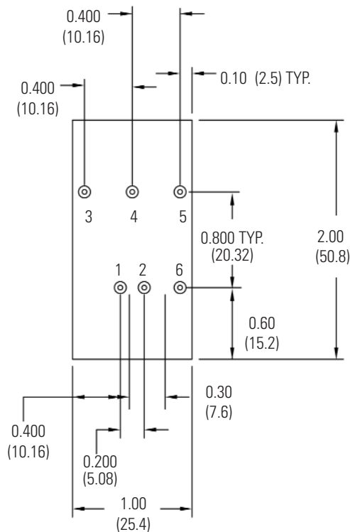
BOTTOM VIEW
