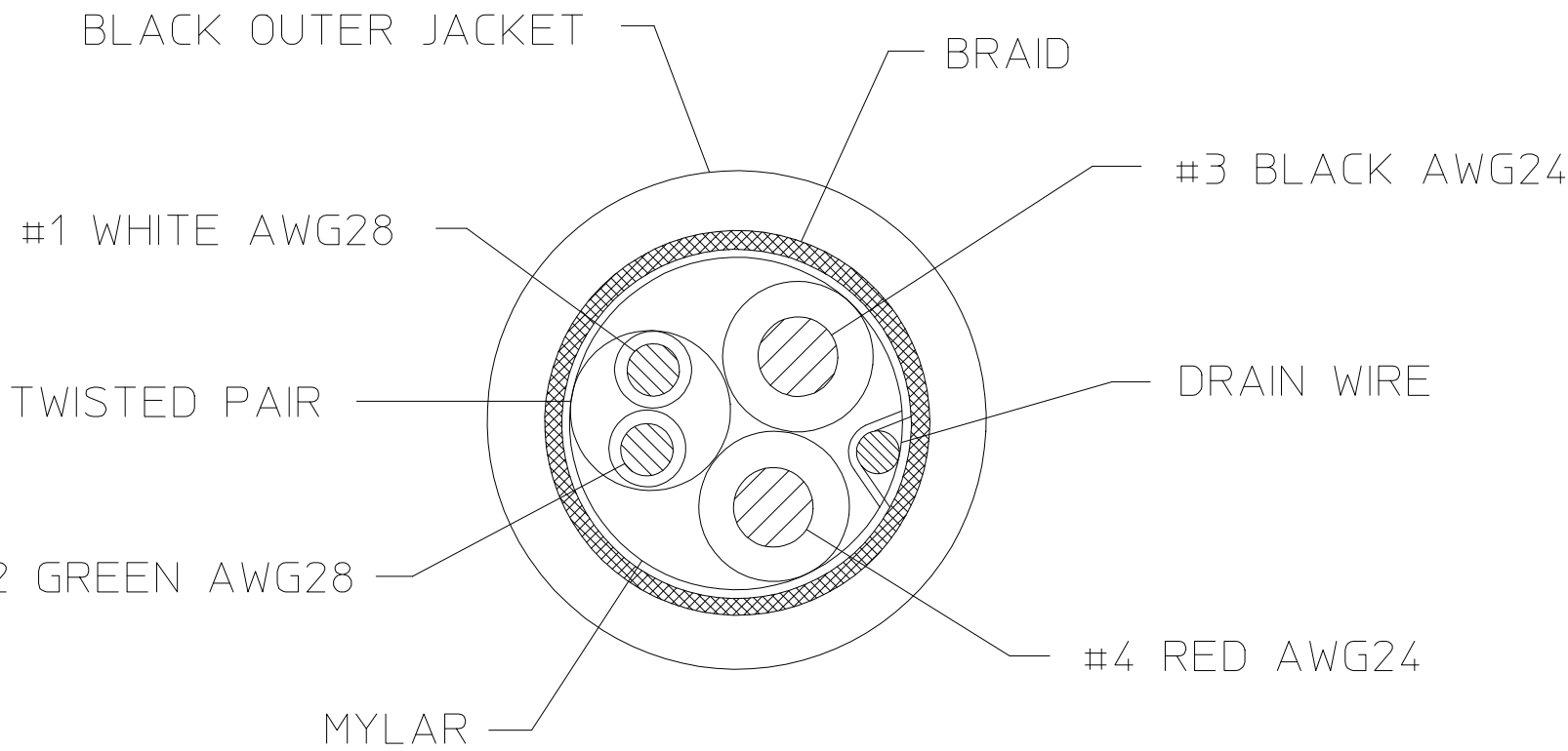
CABLE CONSTRUCTION USB 2.0
