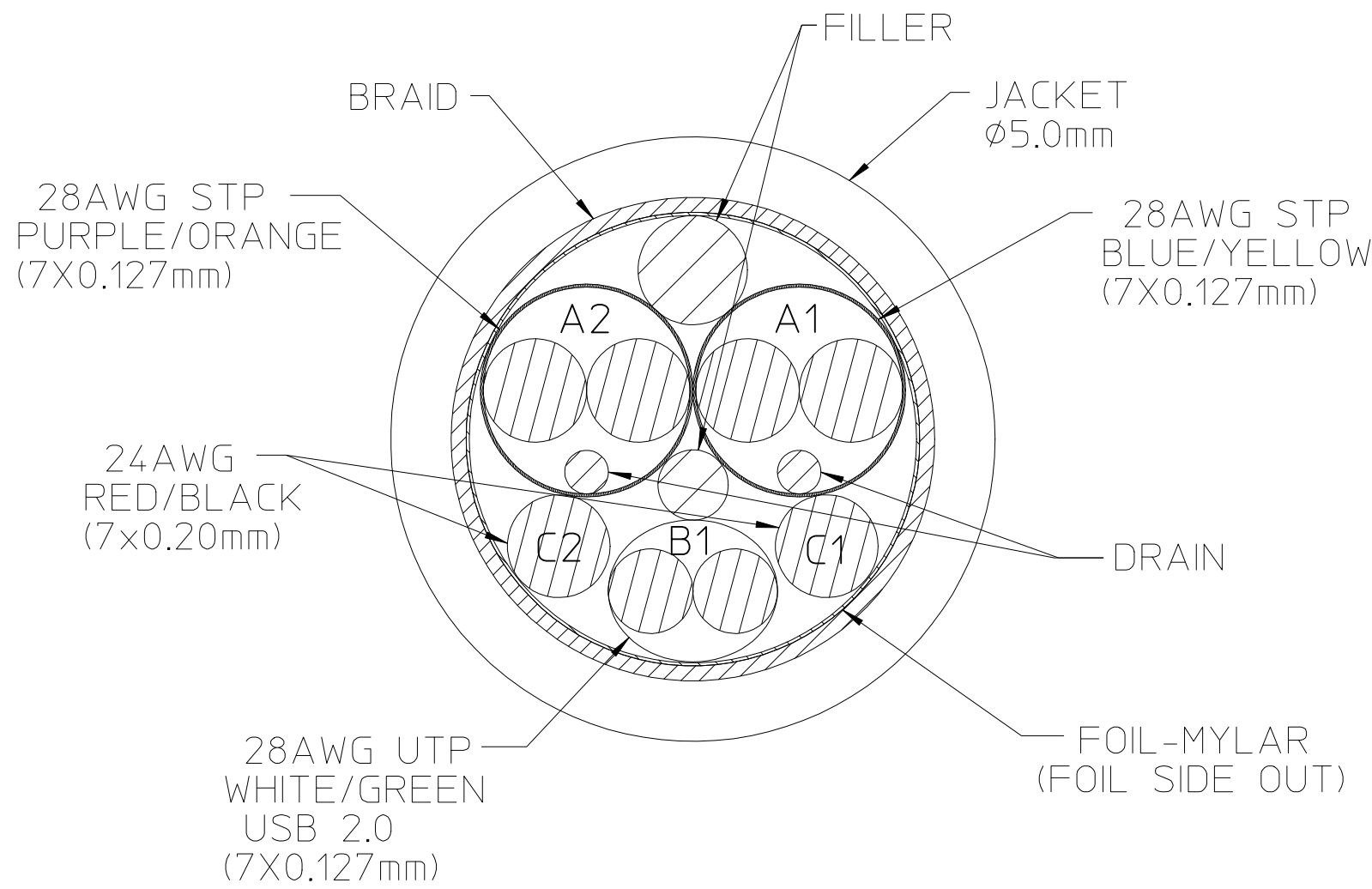
CABLE CONSTRUCTION USB 3.0
