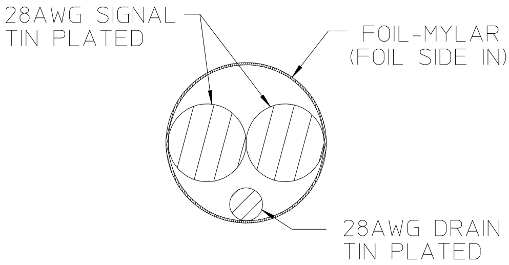
SHIELDED TWISTED PAIR
