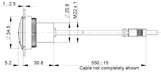
Dimensioned drawing
