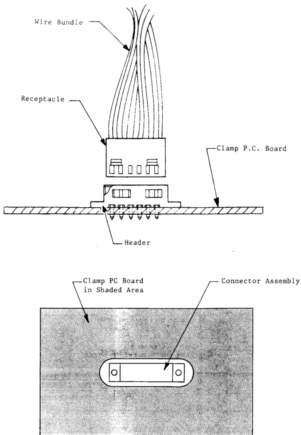
Figure 7 Mounting and Clamping Location for Vibration and Physical Shock
