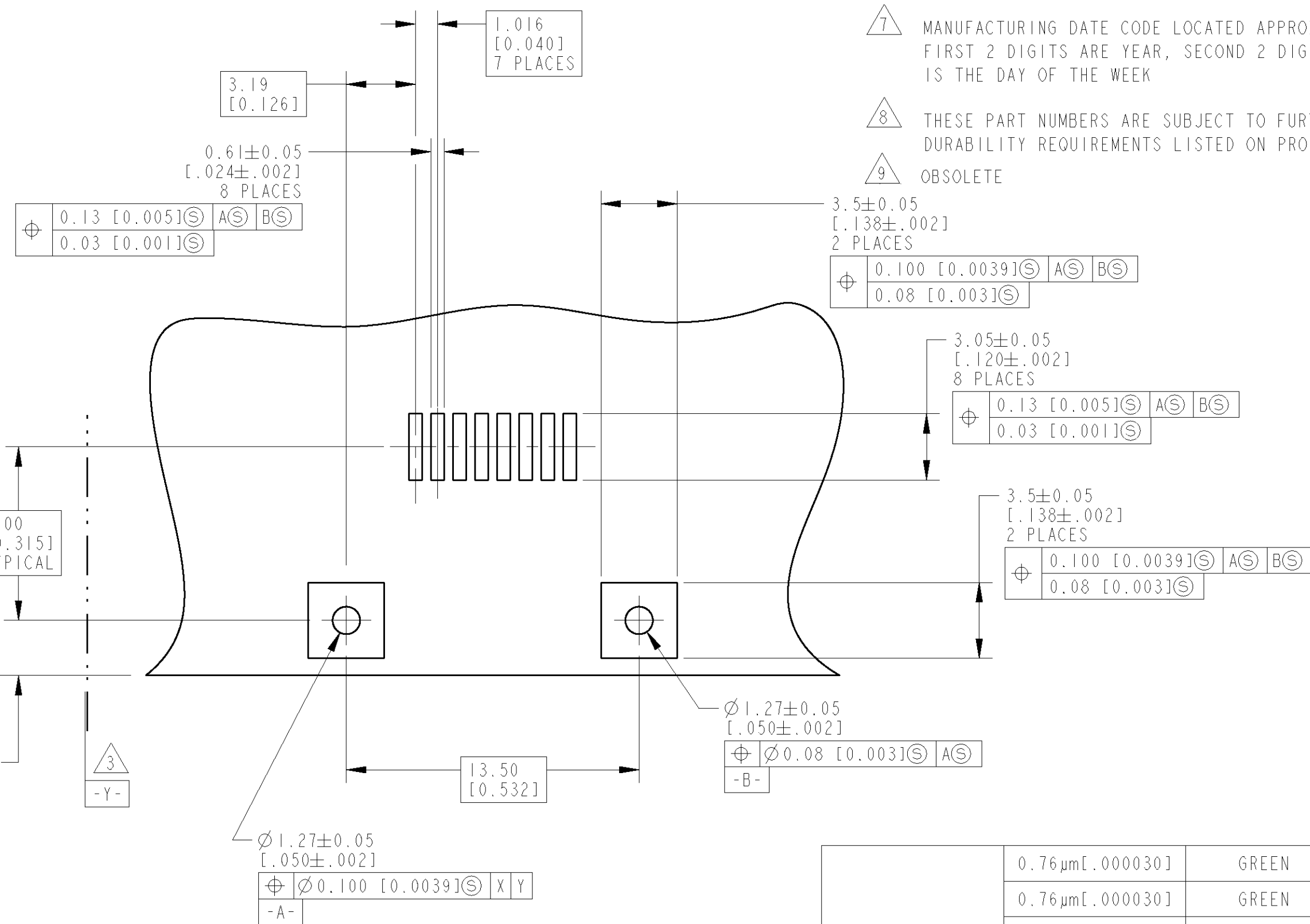
RECOMMENDED PRINTED CIRCUIT BOARD LAYOUT COMPONENT SIDE SCALE 5:1
