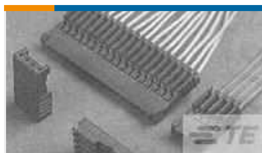
TE Model / Part #1-281786-2 PLUG HE14 IDC 180 12 P AWG 28-26
