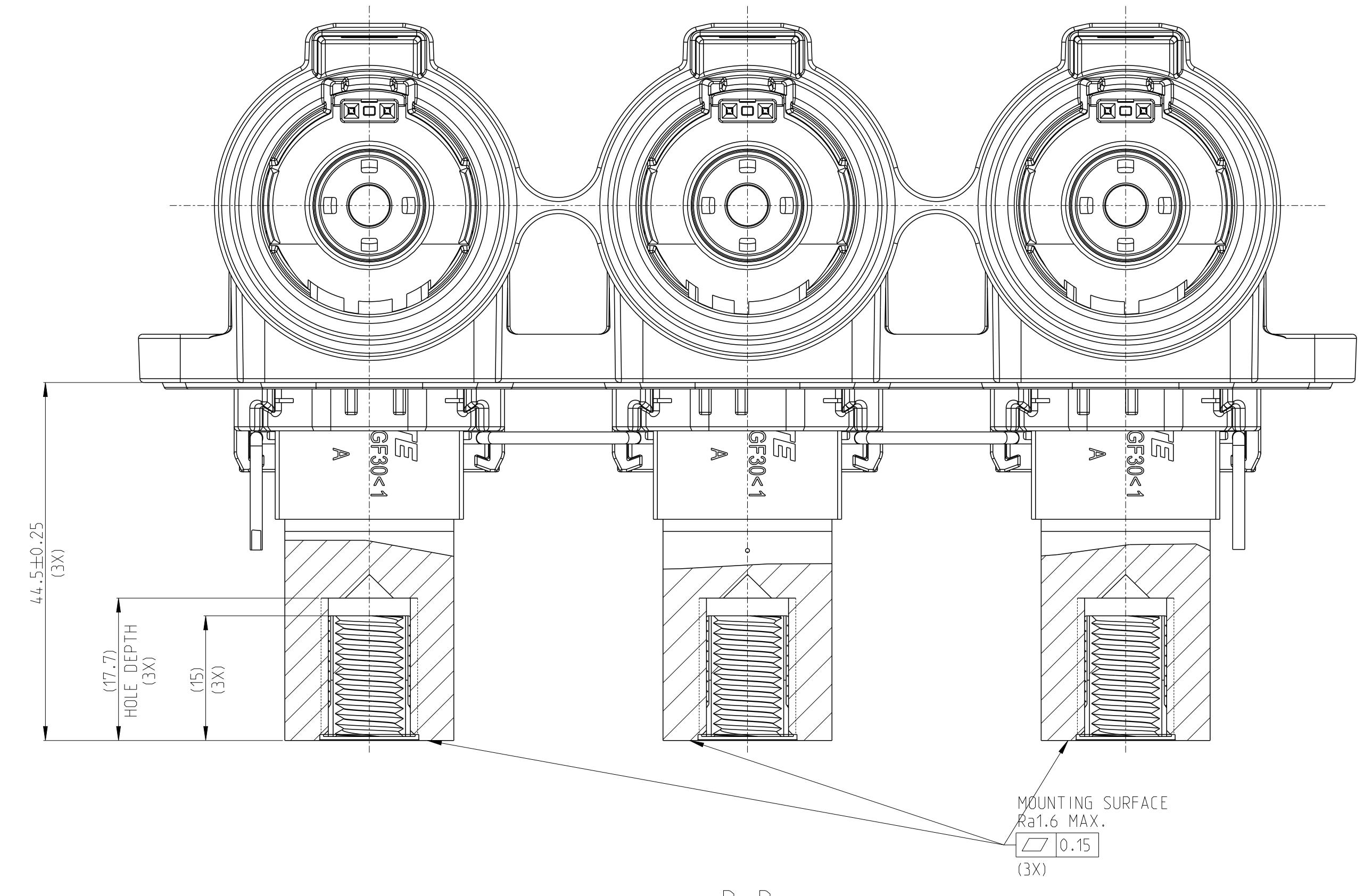
SECTION B-B
