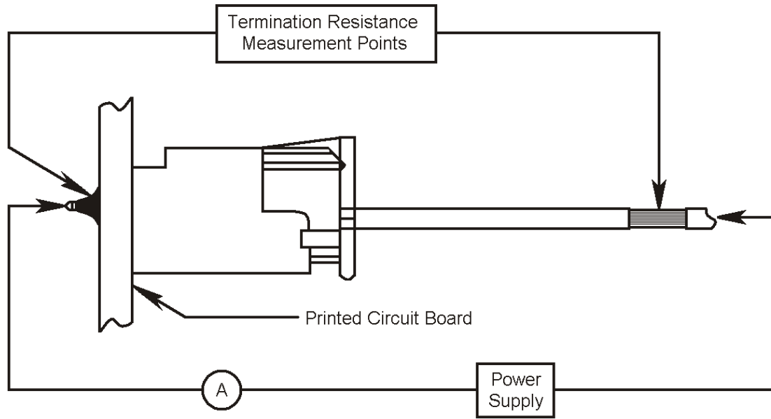
Figure 3 LLCR Measurement Points (Subtract wire bulk)
