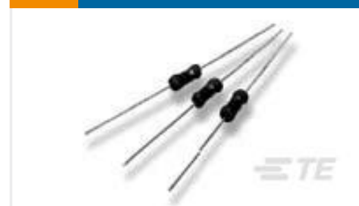
TE Part #4-1625885-0 1W SM M/OX 5% 1R5
