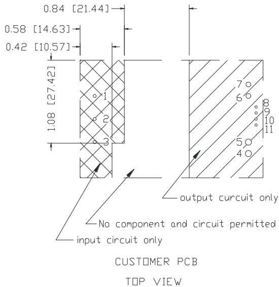
Figure 33. Recommended Pad Layout-1
