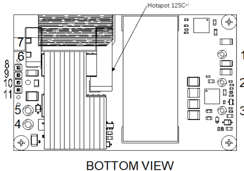
Figure 22. Module Bottom View hot spot
