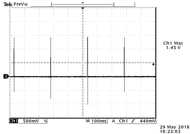
Figure 21. Over current protection Vin = 54V @ Ta = 25°C; CH1: Output Voltage
