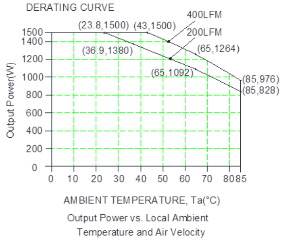
Figure 26. For 0RQP-X5M12P + External heatsink
