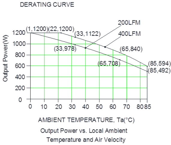
Figure 25. For 0RQP-X5M12P
