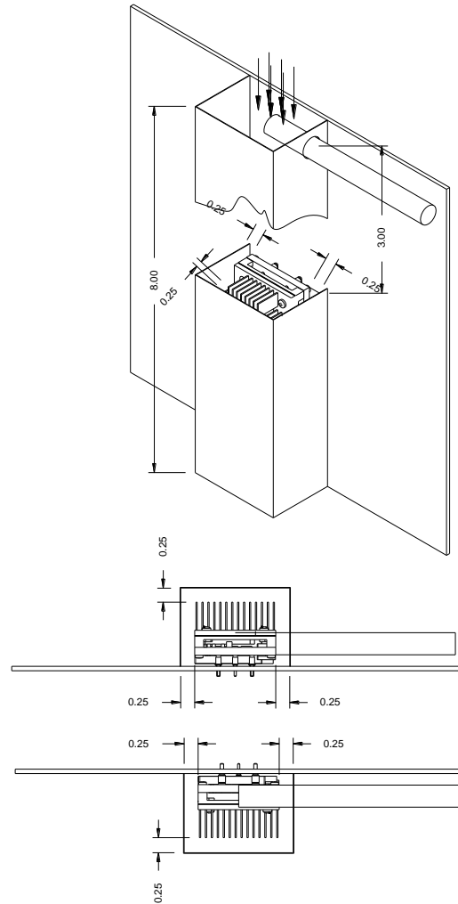
Figure 24. 0RQP-X5M12P + External heatsink
