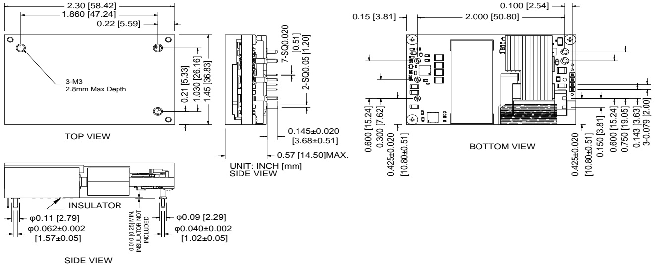
Figure 32. Mechanical Drawing
