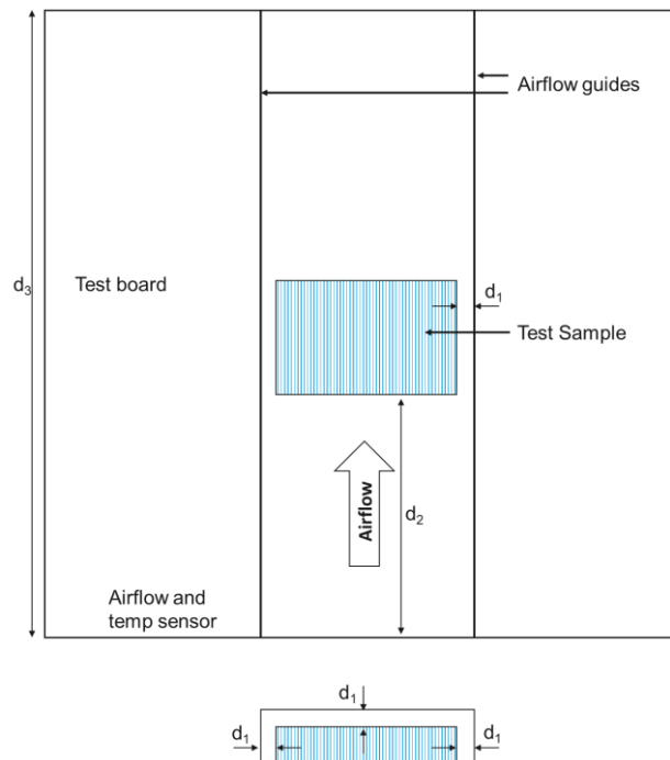
Figure 23. Thermal test setup, Airflow from V_{o-} to V_{o+}
