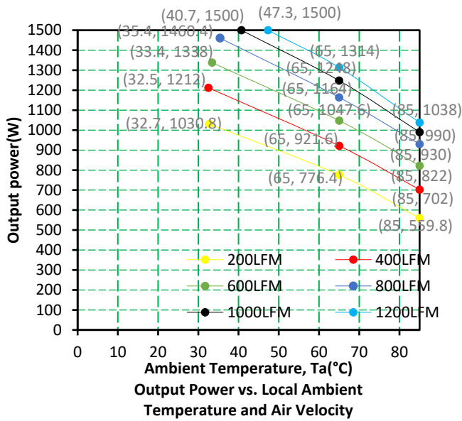
Figure 24. ORQP-X5M12D Vin = 48 V Airflow from V 0 to V IN
