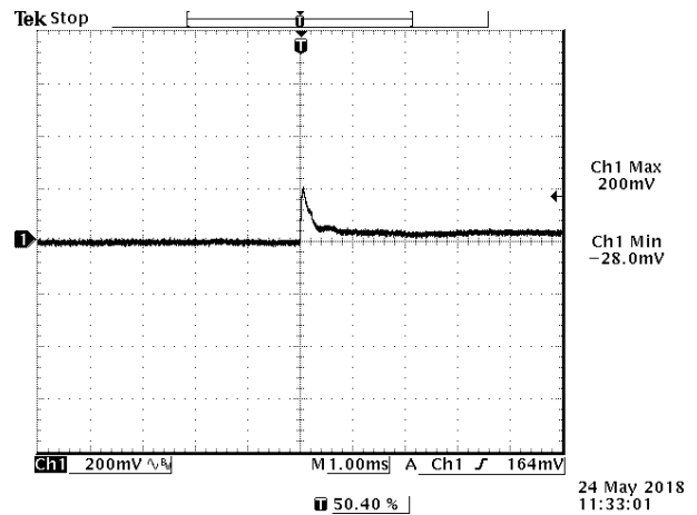
Figure 12. 75%-50% Load, Transients at V_{in}=54V @ T_a=25^{\circ}C
