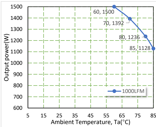
Figure 28. ORQP-X5M12W Vin = 48 V Airflow from Vo- to Vo+
