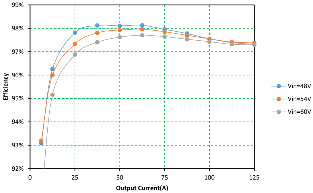
Figure 2. Efficiency data
