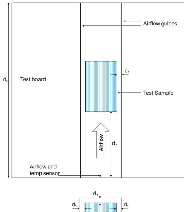
Figure 22. Thermal test setup, Airflow from V_0 to V_{IN}
