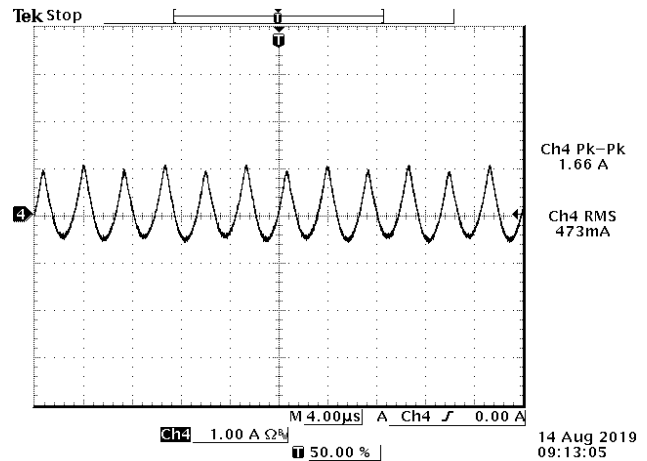
Figure 15. ic (input terminal ripple current), AC component
