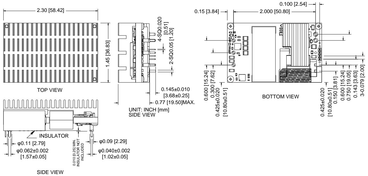
Figure 34. 0RQP-X5M12D mechanical drawing
