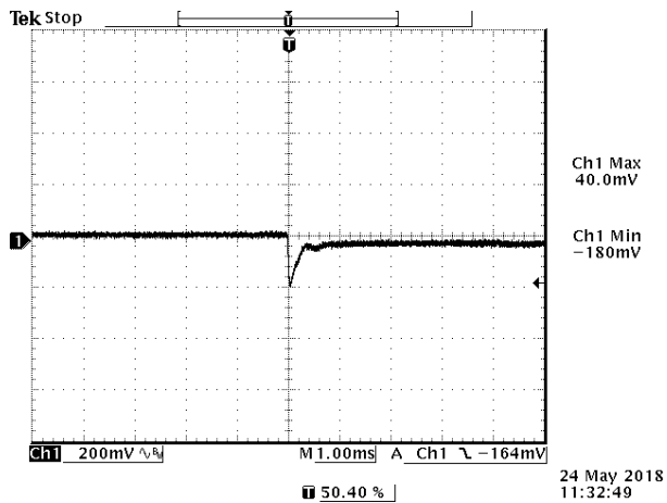
Figure 11. 50%-75% Load, Transients at V_{in}=54V @ T_a=25^{\circ}C
