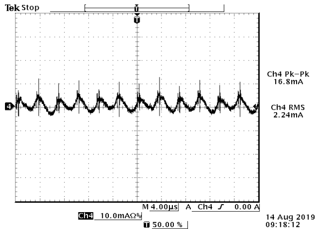
Figure 14. is (input reflected ripple current), AC component
