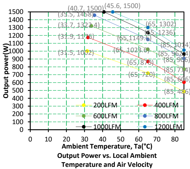
Figure 26. ORQP-X5M12D Vin = 56 V Airflow from V 0 to V IN
