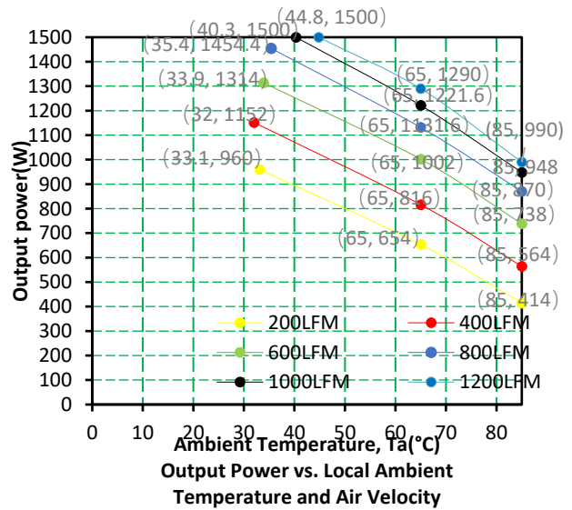
Figure 27. ORQP-X5M12D Vin = 60 V Airflow from V 0 to V IN
