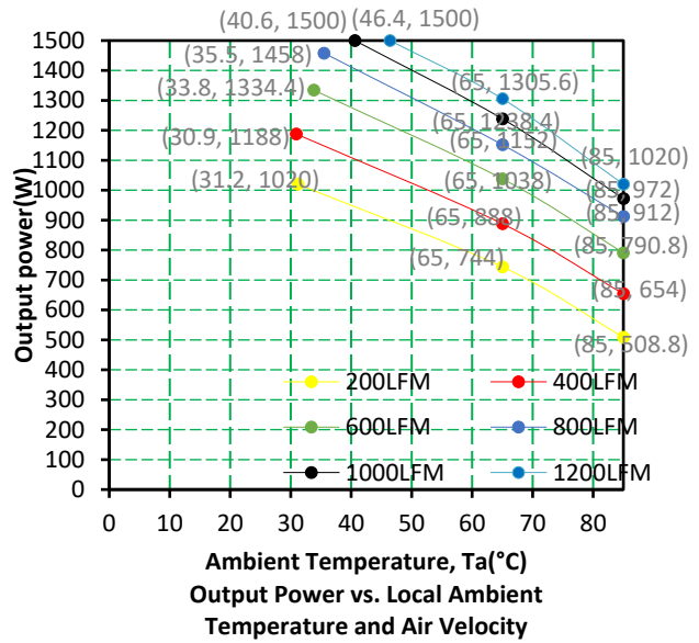
Figure 25. ORQP-X5M12D Vin = 54 V Airflow from V 0 to V IN
