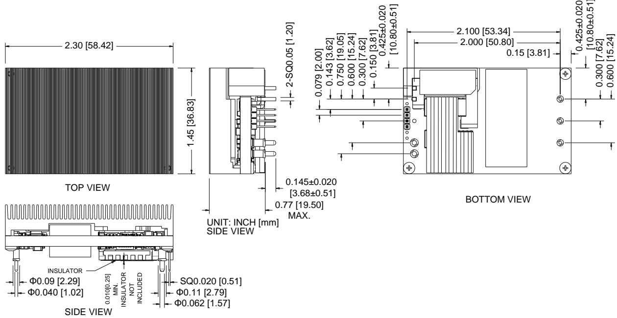
Figure 35. ORQP-X5M12W mechanical drawing
