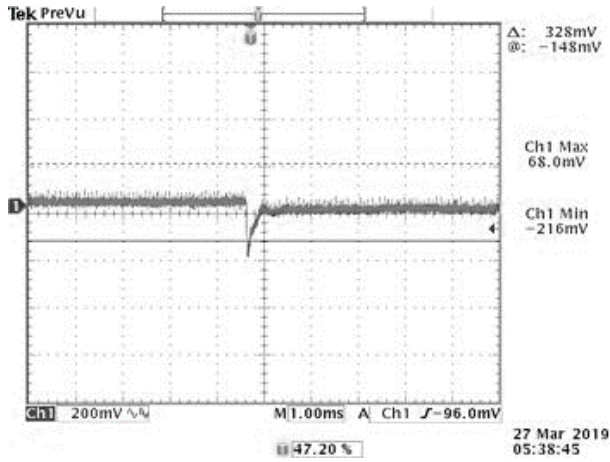
Figure 9. 50%-75% Load, Transients at V_{in}=54V @ T_a=25^{\circ}C
