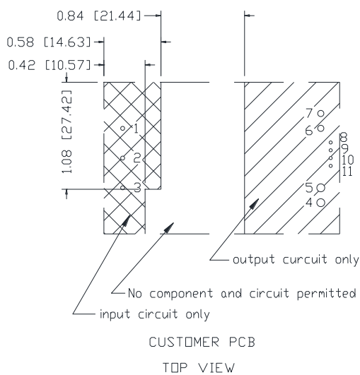
Figure 36. Recommended pad layout-1
