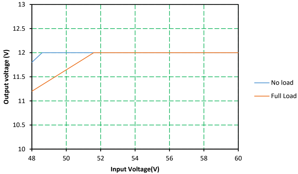
Figure 1. Output Plot vs Input
