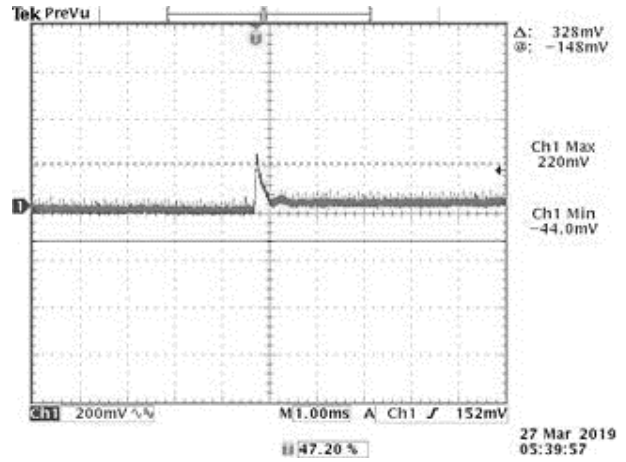
Figure 10. 75%-50% Load, Transients at V_{in}=54V @ T_a=25^{\circ}C
