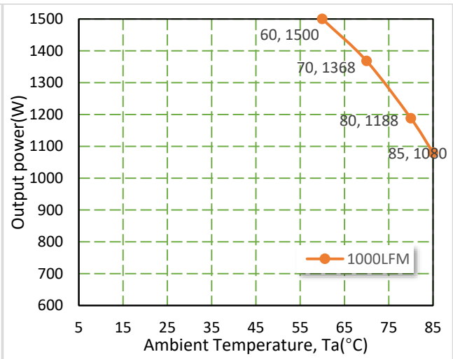
Figure 29. ORQP-X5M12W Vin = 60 V Airflow from Vo- to Vo+
