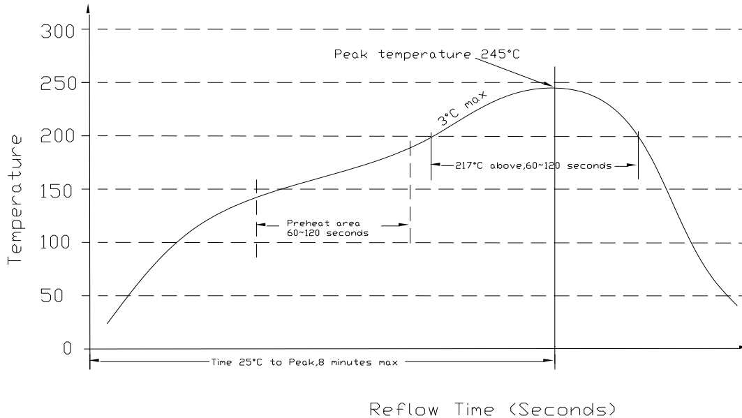
Figure 33. Soldering temperature
