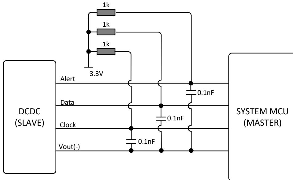
Figure 32. Power management bus application circuit
