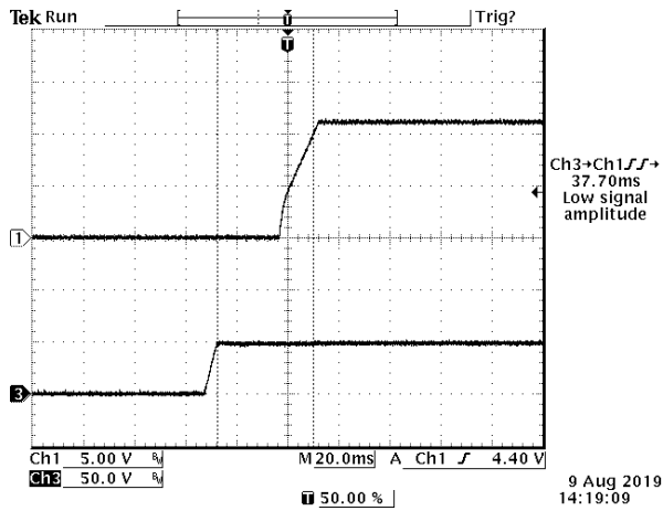
Figure 17. Startup from Vin; Ch1: Vo; Ch3: Vin
