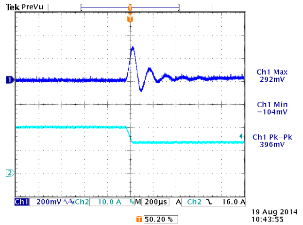
Figure 8. V_{out} = 12\text{ V} , 75%-50% Load Transients
