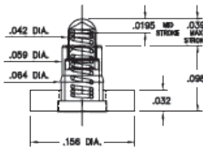
0990-0-50-20-76-14-11-0 Short stroke, Surface mount, Large base
