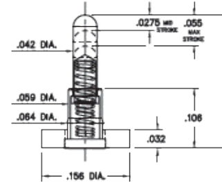
0990-X-50-20-7X-14-11-0 Standard stroke, Surface mount, Large base
