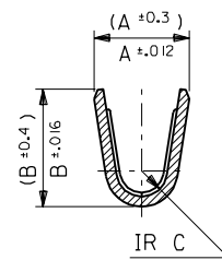
SECTION G-G
