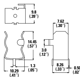
106 001 Device Dimensions
