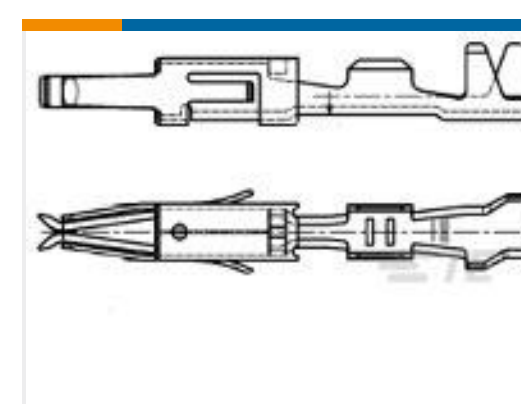
TE Part # 963711-2 MICRO TIM RECEPTACLE CONTACT
